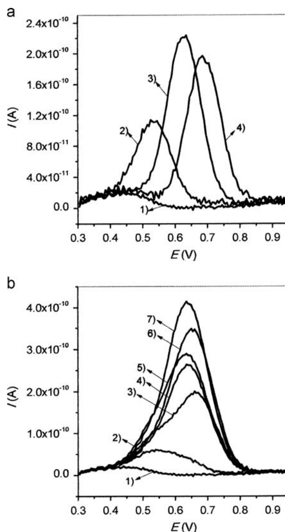
Fig. 1. (a) Square wave voltammograms recorded for: (1) the blank solution; (2) \alpha , (3) \gamma , and (4) \delta tocopherols at a CF disk UME ( \phi = 11 \mu\text{m} ) in Bz/EtOH (1:2)+0.1 mol L -1 H 2 SO 4 . Tocopherol concentrations: 1.2 \times 10^{-4} mol L -1 . \delta E_{\text{SW}} = 0.050 V, \delta E_s = 0.005 V, f = 25 Hz. (b) Square wave voltammograms recorded for some mixtures of tocopherol of different concentrations used in calibration sets: (1) blank, (2) sample 5, (3) sample 11, (4) sample 14, (5) sample 23, (6) sample 18, and (7) sample 24 (see Table 1). Other experimental conditions are the same that those of Fig. 1a.
