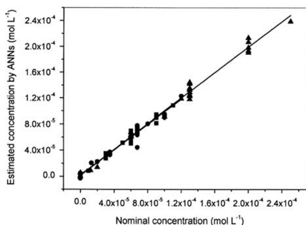
Fig. 4. Dependence between nominal and ANNs calculated concentrations for each substrate. (■) \alpha , (●) \gamma , and (▲) \delta tocopherols.
