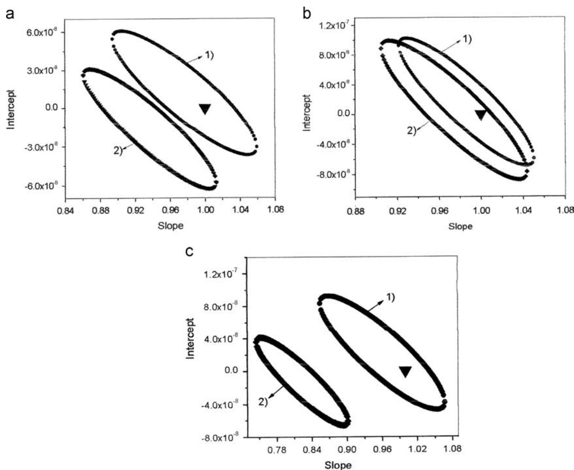
Fig. 6. Elliptical regions of the joint confidence obtained by (1) ANNs, and (2) MCR-ALS methods for (a) \alpha , (b) \gamma , and (c) \delta tocopherols. ( \blacktriangledown ) is the ideal point, (1,0).
